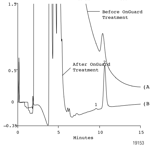
Figure 3. Determination of perchlorate at 0.5 µg/L before (A) and after (B) using Dionex OnGuard sample pretreatment.
