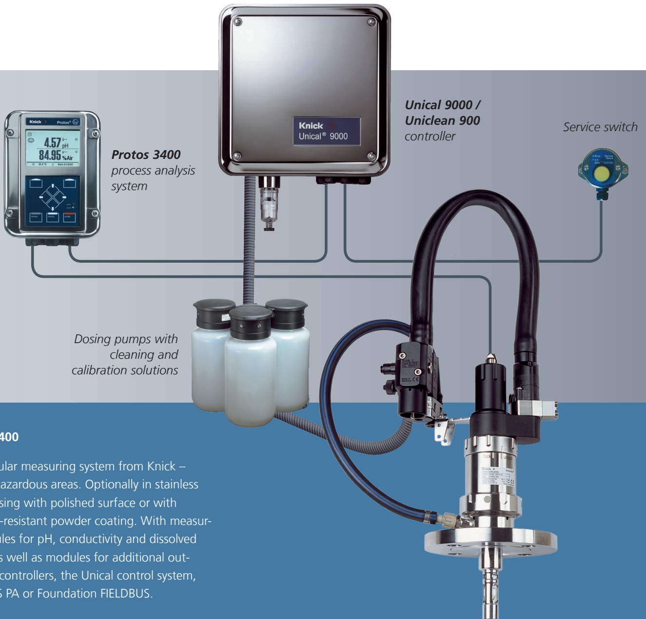
SensoGate WA 130 / WA 130H / WA 132 (PTFE) retractable fitting with pH sensor
