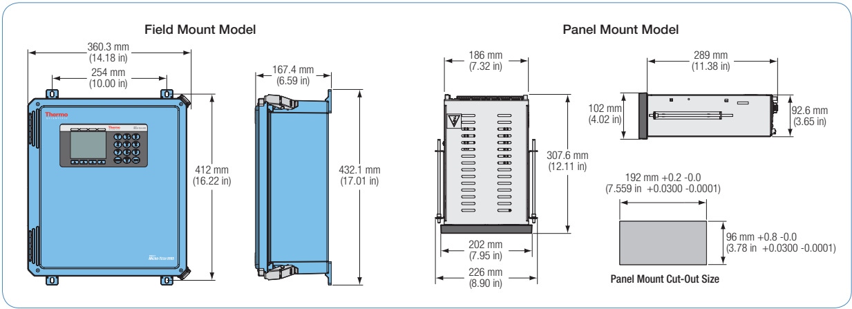
Ramsey Micro-Tech 9105 Impact Weigher Electronics
