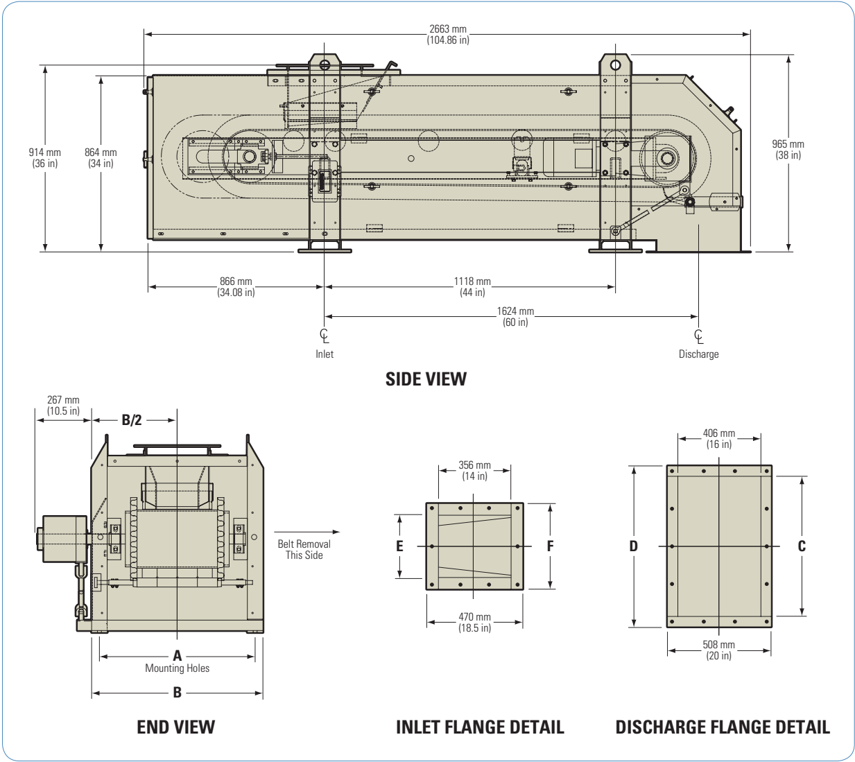
Ramsey Model 90-125 Mid-Range Weighbelt Feeder — Variable Dimensions
