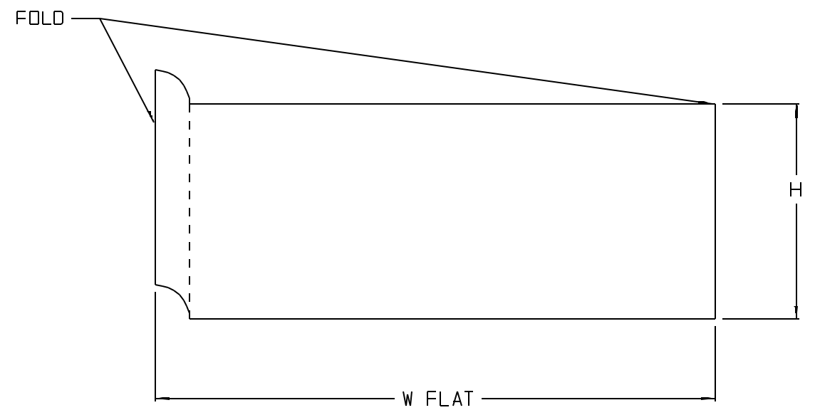
SLEEVE ILLUSTRATION NO SCALE
